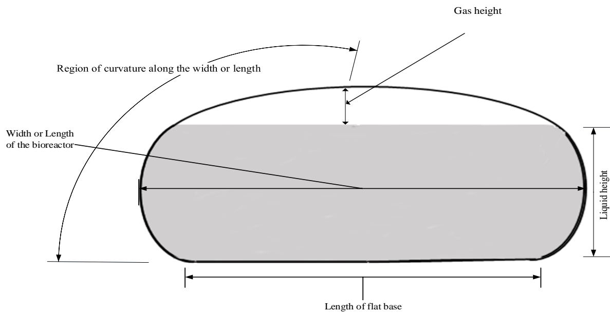
Figure 1. The geometry of a collapsible tank
