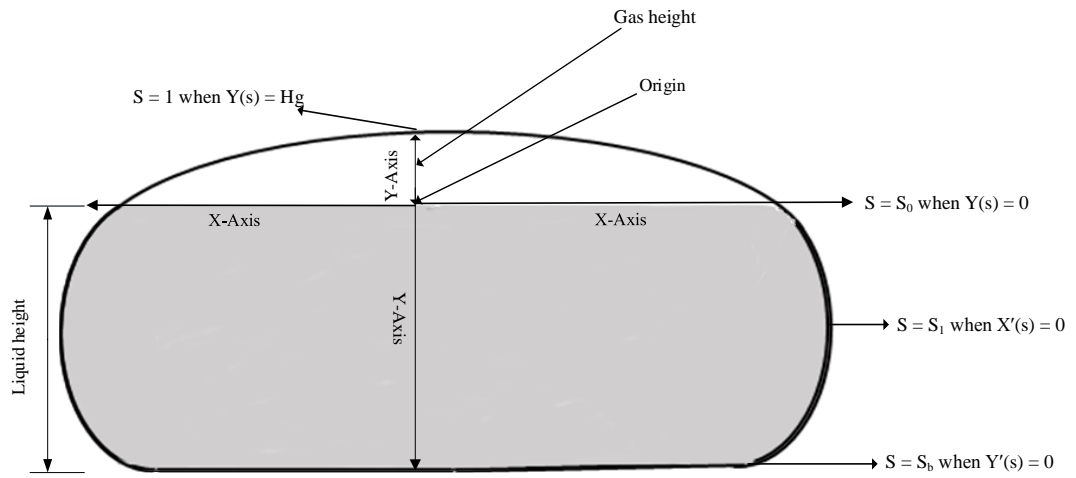
Figure 2. The reference frame used to analyse the collapsible tank
